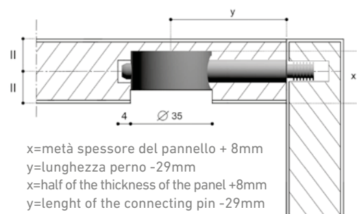
perni M8 / M8 connecting pins
